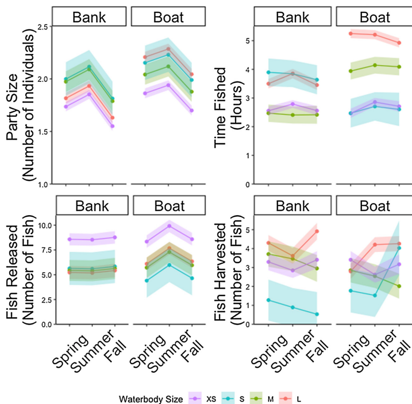
Fig. 2. Spatial (waterbody size) and temporal (season) behavioral patterns between bank and boat anglers for party size (number of anglers), time fished (hr), fish released (number of fish released), and fish harvested (number of fish harvested) using data collected at 29 Nebraska waterbodies during 2007–2017 (Table 1). Angler behavioral patterns from the most supported model for each attribute (Table 4) are presented using the R ggplot2 package (R Development Core Team, 2014; Wickham, 2016) that includes model estimates (dots), directionality (lines), and standard error (ribbons).
