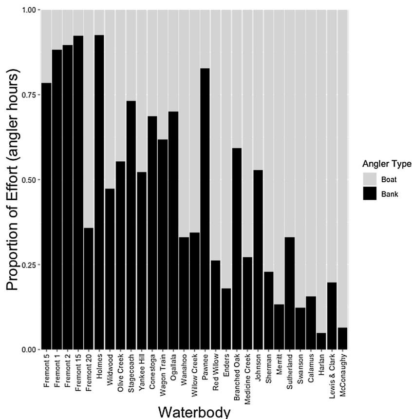
Fig. 1. Proportion of estimated effort (angler hours) for bank and boat anglers across 29 Nebraska waterbodies during 2007–2017. Angler effort was collected from onsite surveys using a stratified multistage sampling regime (Malvestuto, 1996; Kaemingk et al., 2018). Waterbodies are arranged from smallest (left) to largest (right) surface area.
